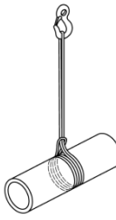
Figure C.1 – Élingage bagué double
