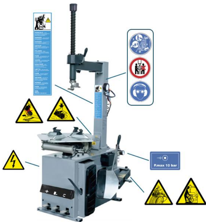
Fig.1-3 Machine color not contractual
