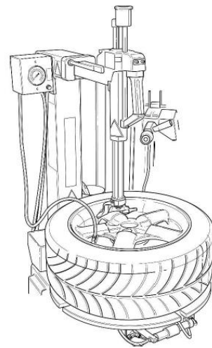
Fig. 4-4-1 Tightening the wheel with the tool
